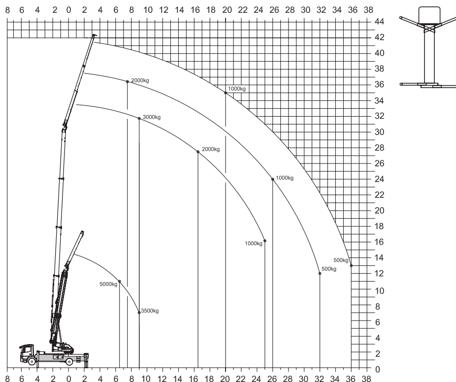
Praca z podestem (HA 3/300)
