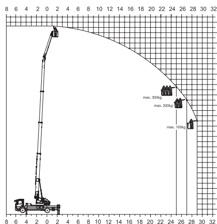
Praca z podestem (HA 3/300)
